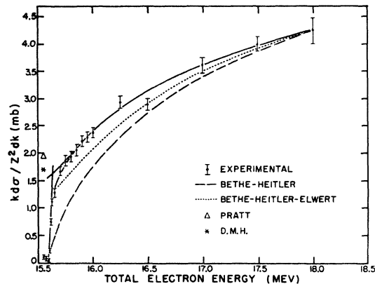
FIG. 13. Comparison of experimental and calculated values of kd\sigma/Z^2dk . The experimental points are normalized to the Bethe-Heitler calculation at 18.0-MeV total energy. The two values at the extreme left represent the tip values as calculated by inverse photoeffect by Pratt and an evaluation of the tip cross section by Deck, Mullin, and Hammer.
