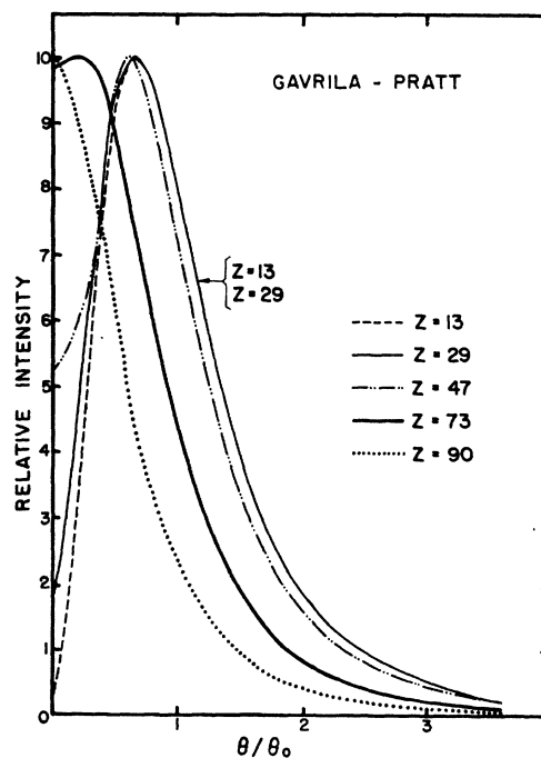
FIG. 3. The angular distributions of photoelectrons, or of tip bremsstrahlung, using the angular distributions of Gavrila weighted according to the contributions to the total yield as calculated by Pratt.
